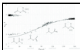
Fig. 4. Plot of \text{S}\cdots\text{O} distance ( d_{\text{SO}} ) against absolute value of \text{S}=\text{C}\cdots\text{C}=\text{O} torsion angle ( |\varphi_{\text{SCCO}}| ) for 739 structures containing \text{CC}(=\text{O})\text{NC}(=\text{S})\text{N} fragment found in CSD 5.32 (Allen, 2002). Title compound is marked with cross. Solid line represents theoretical relation (see: comment).
