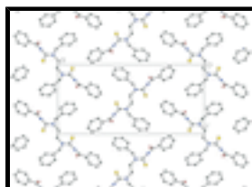
Fig. 3. Tiling of ladders seen along [100] direction. Hydrogen atoms have been omitted for clarity.
