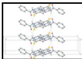
Fig. 2. Ladder-like structural motif found in the structure of the title compound. Hydrogen bonds are shown as dashed lines. C-bonded hydrogen atoms have been omitted for clarity.
